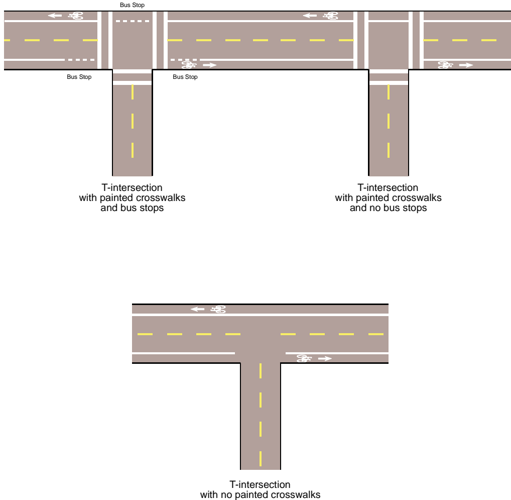
Figure 8. Typical Bike Lane Striping at T-intersections
