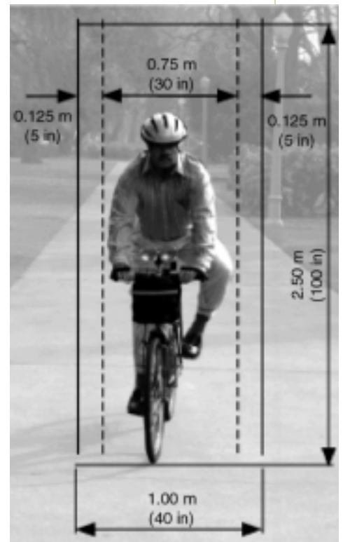
Figure 1. Bicyclist Operating Space
